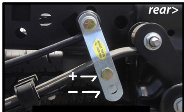
Select pre-load and ride height
